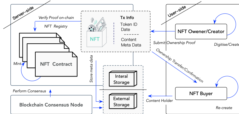
Fig. 1: Model of NFT Systems
